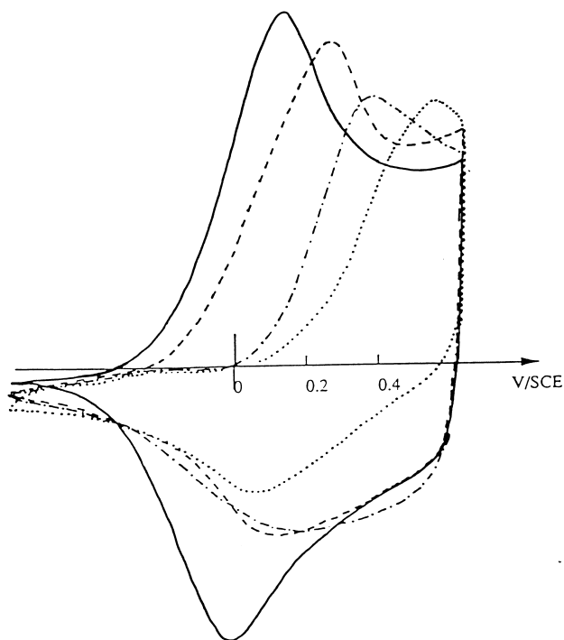
Fig. 4. Cyclic voltammograms on Pt of poly( 10b ) in 0.1M \text{Bu}_4\text{NClO}_4 + \text{CH}_3\text{CN} in the presence of increasing \text{NaClO}_4 concentration: 0M (—); 10^{-5}\text{M} (---); 10^{-3}\text{M} (- · -); 10^{-2}\text{M} (· · ·). The film was electrosynthesized at 0.9 V (vs SCE) in 0.5M \text{Bu}_4\text{NClO}_4 + \text{CH}_3\text{CN} containing 0.1M of 10b (deposition charge, 500 \text{ mC cm}^{-2} ). Scan rate, 20 \text{ mV s}^{-1} . (Reprinted from Korri-Youssefi et al. [66], copyright 1994, with permission from Elsevier Science.)
